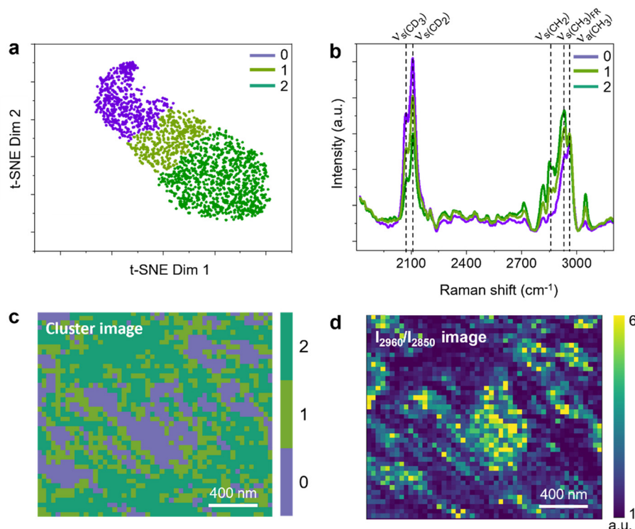
Fig. 3 (a) t-SNE dimension plot of the first five PCs obtained from the hyperspectral TERS image of \text{d}_{62} -DPPC:DOPC monolayer presented in Fig. 2. (b) TERS spectra corresponding to the clusters 0 (purple), 1 (light green) and 2 (dark green) in panel a. (c) TERS intensity image of the clusters 0 (purple), 1 (light green) and 2 (dark green). (d) TERS image of the I_{2960}/I_{2850} ratio.
