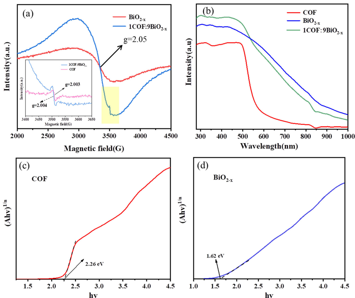
Fig. 4 (a) EPR spectra of \text{BiO}_{2-x} , the \text{COF} and the \text{1COF:9BiO}_{2-x} catalyst; (b) UV-vis absorption spectra of the \text{COF} , \text{BiO}_{2-x} and the \text{1COF:9BiO}_{2-x} composite; and (c and d) energy band gaps of the \text{COF} and \text{BiO}_{2-x} .
