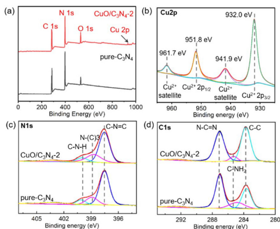
Fig. 4 (a) XPS survey spectra of pure C_3N_4 and CuO/C_3N_4-2 . (b) High-resolution Cu 2p XPS spectra of CuO/C_3N_4-2 . High-resolution XPS spectra of (c) N 1s and (d) C 1s of pure C_3N_4 and CuO/C_3N_4-2 .
