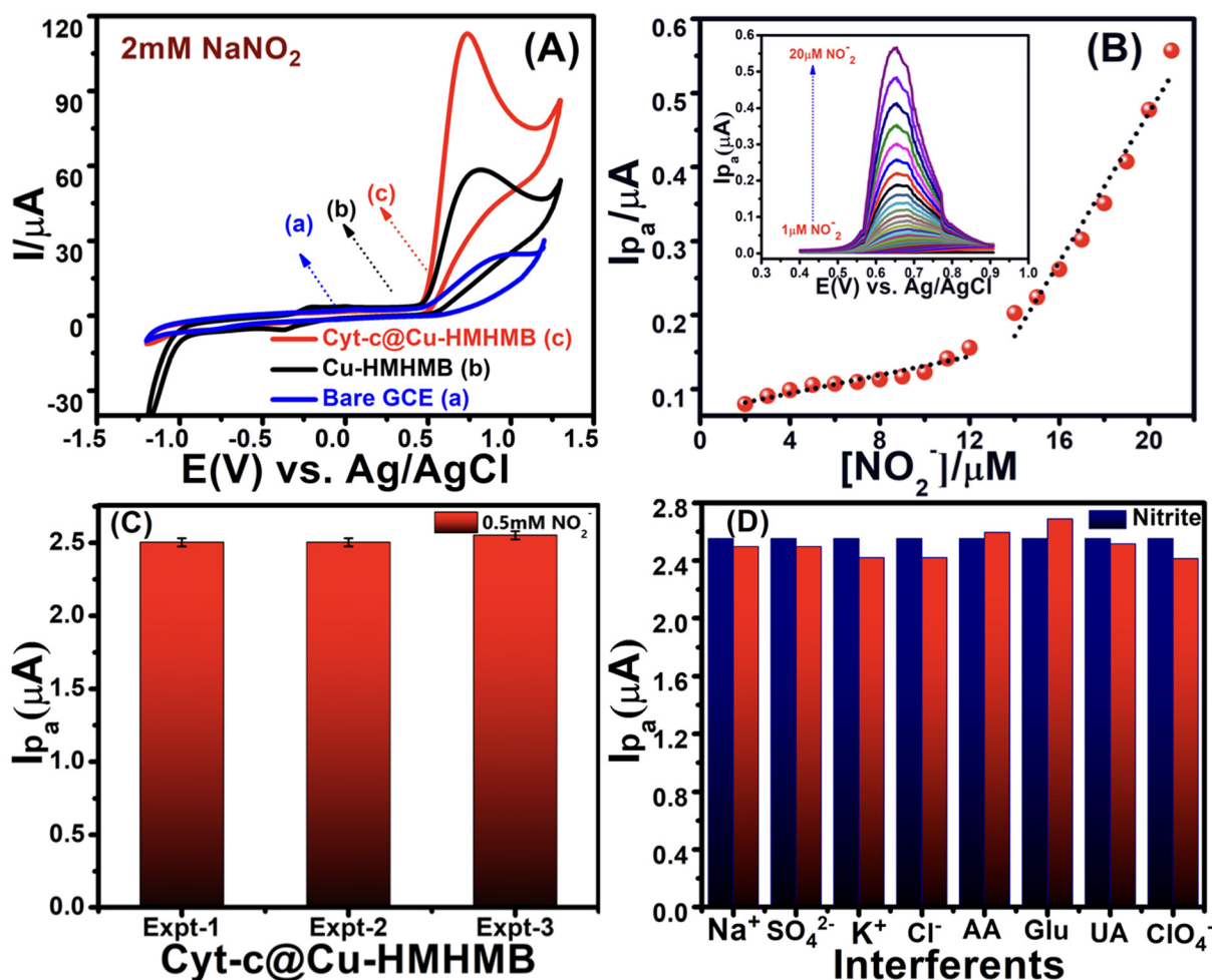
Fig. 3 CVs recorded for 2 mM \text{NaNO}_2 over the bare GCE (a), Cu-HMHMB/GCE (b) and Cyt-c@Cu-HMHMB/GCE (c) in 0.1 M phosphate buffer solution (pH = 7.2) at a scan rate of 50 \text{ mV s}^{-1} [panel A]. DPVs recorded for changing concentrations of nitrite ( \text{NO}_2^- ) in 0.1 M PBS (pH 7.2) over Cyt-c@Cu-HMHMB/GCE [inset, panel B]. Calibration plots between I_p vs. [\text{NO}_2^-] with two linear ranges from 1 \text{ }\mu\text{M} to 12 \text{ }\mu\text{M} , I_p = 3.112 + 0.7072 [\text{NO}_2^-] , ( R^2 = 0.98 ) and from 13 \text{ }\mu\text{M} to 20 \text{ }\mu\text{M} , I_p = -26.69 + 5.0393 [\text{NO}_2^-] , ( R^2 = 0.97 ) [panel B]; reproducibility of the Cyt-c@Cu-HMHMB/GCE electrode system for the electro-detection of the same concentration (0.5 mM) of nitrite ions in 0.1 M PBS (pH 7.2) recorded via DPV measurements over three prepared electrode systems [panel C]; interference study of inorganic compounds and biomolecules on the current response of 0.5 mM nitrite ions in 0.1 M phosphate buffer solution (pH = 7.2) over the Cyt-c@Cu-HMHMB/GCE bio-composite [panel D].
