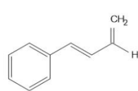
Cinnamaldehyde
