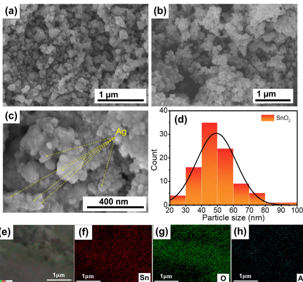
Fig. 2 SEM images of (a) \text{SnO}_2 and (b and c) Ag TNPs/ \text{SnO}_2 ; (d) particle size distribution histogram of \text{SnO}_2 in the Ag TNPs/ \text{SnO}_2 sample; (e-h) SEM-EDS elemental mapping of Ag TNPs/ \text{SnO}_2 .
