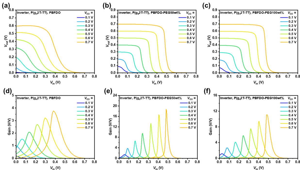
Fig. 6 OECTs-based complementary inverters. The voltage transfer characteristics and gain of inverters based on P(g 4 2T-TT) with different n-type channel materials (a) and (d) PBFD0, (b) and (e) PBFD0-PEG50wt%, (c) and (f) PBFD0-PEG100wt%.
