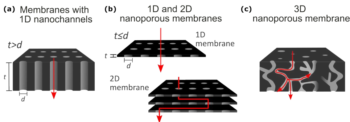
Figure 2. Illustrations of the solid-state membrane film structures included in our review: (a) 1D nanochannels with a longer channel length (or film thickness, t ) than the diameter ( d ) of the nanopores; (b) 2D membrane thin films with 1D nanopores where d > t or the stacks of such 1D membranes (called 2D membranes); (c) 3D nanoporous membranes with irregularly connected nanopores.
