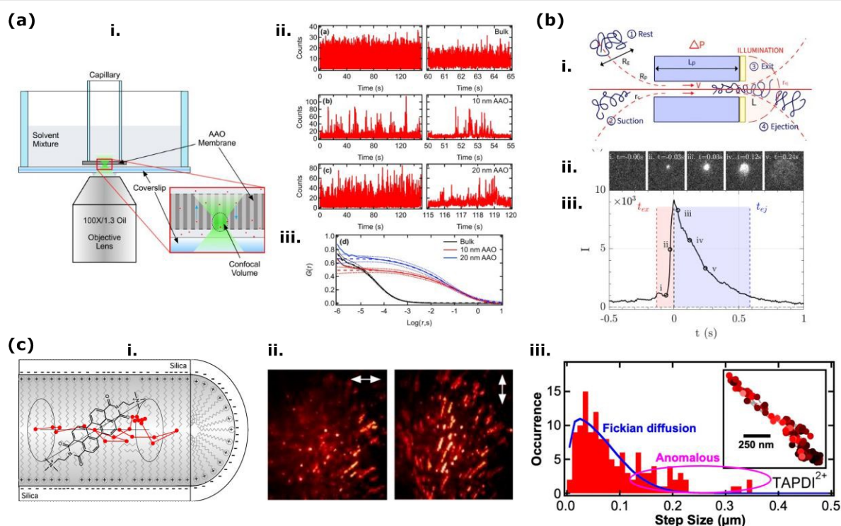
Figure 9 (a) (i) Experimental FCS setup with the expanded view of the AAO membrane. (ii) Representative time transients for RhB in a bulk ethanol solution, ethanol-filled 10 nm AAO nanochannels, and ethanol-filled 20 nm AAO nanochannel, top to bottom, respectively. (iii) Autocorrelation data (solid lines) obtained from the same series of samples based on averages from multiple replicate measurements. Reprinted with permission from ref. 283 . Copyright 2023, American Chemical Society. b) (i) Schematic explaining the translocation mechanism of polymers (also applied for different DNA) through 1D nanochannel. R_g stands for the gyration radius of the polymer coil. (iii) Mean event quantified after averaging all segmented events tracked by single-molecule fluorescence microscopy images (ii). The red region ( t_{ex} ) and blue region ( t_{ej} ) correspond to the time of images captured while the polymer coil exits the nanopore and the coil moves outside the illumination region, respectively. Reproduced from ref. 284 with permission from the Royal Society of Chemistry. (c) (i) Illustration of a cationic PDI molecule inside a CTAB-loaded silica mesopore. (ii) Simultaneously collected Z-projection images of the PDI molecules at two orthogonal polarizations (double-ended white arrows with 3 \mu\text{m} length). (iii) Detected single-molecule trajectory presenting the 1D motion
