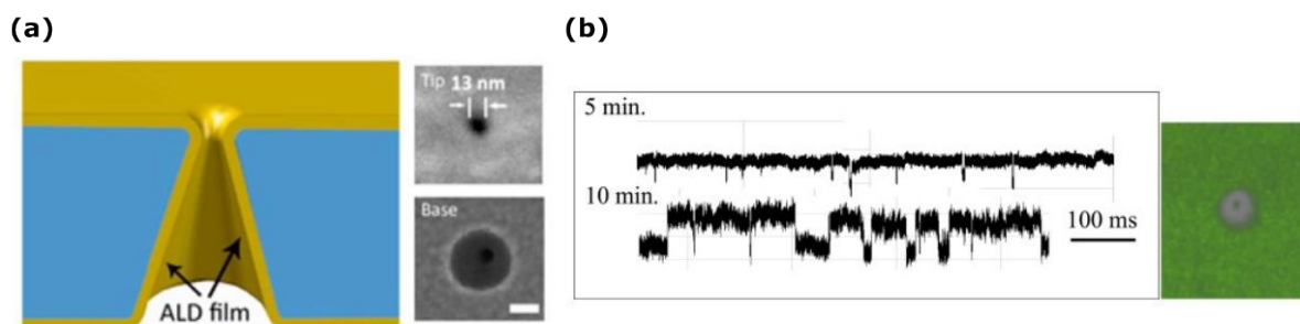
Figure 8. (a) Schematic illustration of uniform ALD coating on a single conical nanochannel and SEM images of the tip and base sides. The scale bar is 100nm. Reprinted with permission from ref. 279 . Copyright 2015, American Chemical Society. (b) (left) Resistive pulse signals of a 1:1 mixture of 22 bp ss-DNA and ds-DNA after 5 min and 10 min. (right) STED super-resolution microscopy image at 30 min. Reprinted from ref. 280 with the permission of AIP Publishing.
