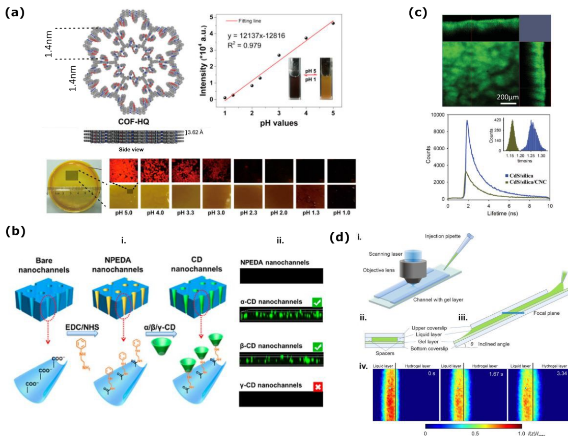
Figure 6. (a) (top-left) Top and side view schemes of 8-hydroxyquinoline-functionalized covalent organic framework (COF-HQ). (top-right) The relation between probed environmental pH and the fluorescence intensity. (bottom) Naked eye visible pH-dependent color changes of the free-standing COF-HQ based matrix membrane. Reprinted with permission from ref. 238 . Copyright 2018, American Chemical Society. (b) i. Schematics of functionalization of the CD-self-assembled nanochannel membranes, ii. The fluorescence confocal microscope images of nanochannel membranes before and after NPEAD modification and CD self-assembly. Reprinted with permission from ref. 202 . Copyright 2020, American Chemical Society. (c) (top) CLSM z-stack image of iridescent, luminescent chiral nematic CdS QD loaded mesoporous silica film presenting the film's (large area) surface and (top and right) cross-section. (bottom) Fluorescent lifetime decays of the CdS/mesoporous films that were fabricated differently and the inset presents corresponding histograms of pixel-by-pixel lifetime distributions of these films. Adapted with the permission from ref. 239 . Copyright 2013, Wiley. (d) (i) bird view of the setup employed for transient molecular transport measurement using inclined microscopic observation; (ii) Cross-sectional view of the channel containing the gel layer; (iii) Side view of the channel with the observed focal plane indicated with a blue line; (iv) Transient permeation of uranine from the upper liquid layer to the lower hydrogel layer. The colored bar shows the normalized fluorescence intensities. Reprinted with permission from ref. 240 . Copyright 2019, Plos One.
