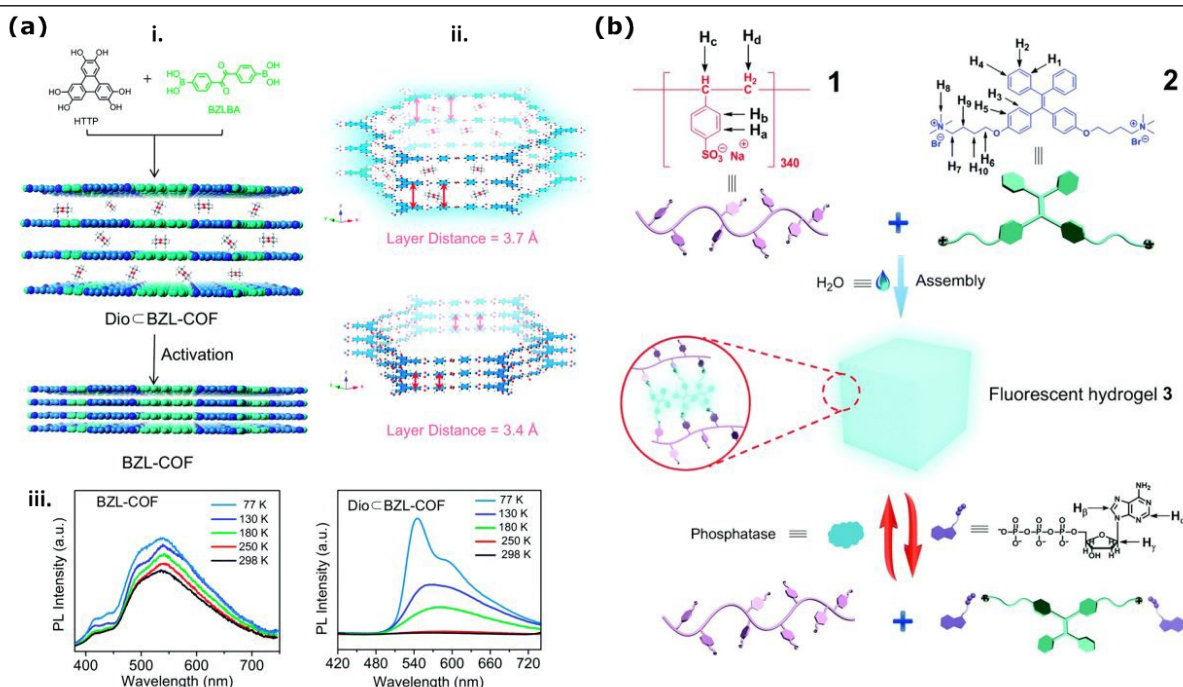
Figure 5. (a) Illustration of COF stacking arrangements and its relation to optical fluorescence emission. (i) Schematics presenting COF activation via decreasing the interlayer distance and influencing the AIE and ACQ (ii) As a factor of decreasing interlayer distance (iii) and the temperature detected phosphorescence emissions increase. Reproduced from ref. 218 with permission from the Royal Society of Chemistry. (b) Chemical structures poly(sodium p-syrenesulfonate) hydrogel (1) and amino-derivative of TPE employed for the synthesis of the hydrogel (2) and the cartoon representation of the formation and bioresponsive reversible properties of the supramolecular fluorescent hydrogel in the presence of BZ ATP (3). Reproduced from ref. 221 with permission from the Royal Society of Chemistry.
