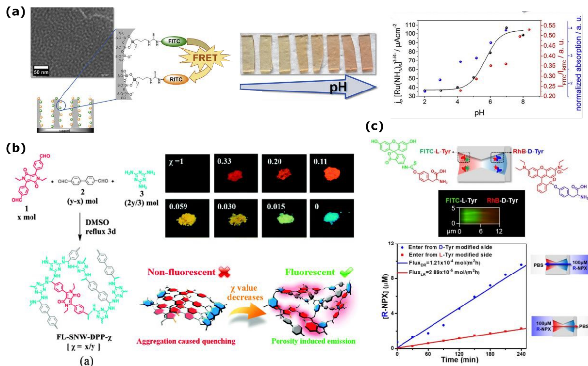
Figure 3. (a) FRET dye pair (FITC, green, donor and RITC, orange, acceptor) functionalized mesoporous silica film changes its fluorescence emission intensity (red spheres in the right graph) as a factor of changing pH. This change agrees with the pH-dependent transport properties of probe molecule [\text{Ru}(\text{NH}_3)_6]^{3-/4-} from electrochemical investigations (black spheres in the right graph). Reprinted from ref. 164 with permission from Elsevier. Copyright 2019, Elsevier. (b) Mixing of 4,40-(2,5-diethyl-3,6-dioxo-2,3,5,6-tetrahydropyrrolo[3,4-c]pyrrole-1,4-diyl)dibenzaldehyde (1) with 4,40-biphenyldicarboxaldehyde (2) and melamine (3) to fabricate different FL-SNW-DPP- \chi type POP membranes where \chi is the molar ratio of (1). Solid-state photographic images of the samples with different \chi taken after placing the samples under UV-lamp ( \lambda=365 nm). Schematic representation of “porosity induced emission” mechanism of the POPs. Adapted with the permission of ref. 165 . Copyright 2015, Rocal Society of Chemistry. (c) (up) The schematic diagram of the asymmetrically modified nanochannel in PET and the fluorescence confocal image of labeled L-Tyr/D-Tyr channels. (bottom) The change of concentration with respect to time during the directional transport of R-NPX. Reprinted with permission from ref. 166 . Copyright 2021, American Chemical Society.
