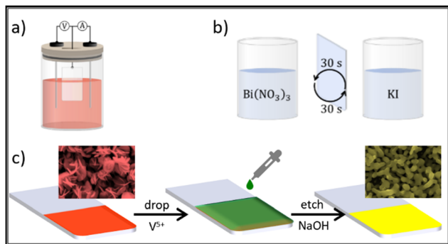
Fig. 12 \text{BiVO}_4 synthesis via \text{BiOI} template through: (a) electrodeposition; (b) SILAR; and (c) drop cast of V precursor for thermal conversion \text{BiOI} \rightarrow \text{BiVO}_4 common to both approaches.
