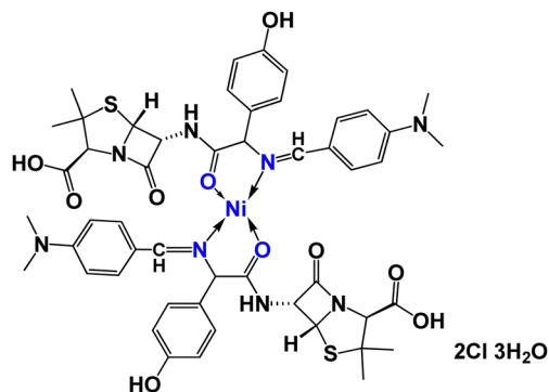
Fig. 1 Structure of [\text{Ni(II)(SB)}_2] \cdot 2\text{Cl} \cdot 3\text{H}_2\text{O} .
