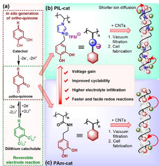
Fig. 32 Construction of catechol-based PIL/CNTs buckypaper for LIBs. (a) ortho -Quinone/diliithium catecholate redox reaction. (b and c) Enhancement in the electrochemical performance of cationic PIL-cat (b) compared to its neutral counterpart PAm-cat (c). Reproduced from ref. 212 with permission from ACS, Copyright [2018].
