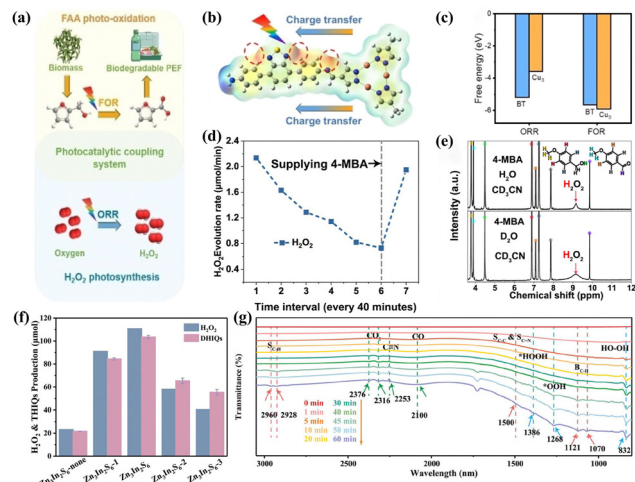
Fig. 8 (a) The schematic representation of \text{H}_2\text{O}_2 photosynthesis coupled with FFA photo-oxidation. 103 (b) Differential charge density diagram of \text{Cu}_3\text{-BT-COF} . 103 (c) Adsorption energy of \text{Cu}_3 and BT units in \text{Cu}_3\text{-BT-COF} for FFA and \text{O}_2 . 103 (d) The \text{H}_2\text{O}_2 production rate of ASCN-3. 102 (e) ^1\text{H} NMR spectra of the different photocatalytic solutions after photocatalysis. 102 (f) The yields of DHIQs and \text{H}_2\text{O}_2 . 101 (g) Time-dependent in situ FTIR spectra of \text{ZnIn}_2\text{S}_6 in THIQ/ \text{CH}_3\text{CN} solution. 101
