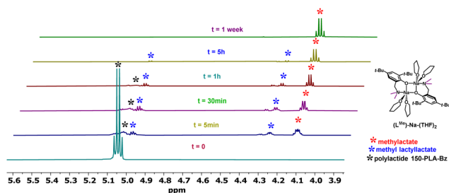
Fig. 13 The PLA degradation process in the presence of ( L^{\text{Me}} )-Na-(THF) 2 monitored by 1 H NMR (C 6 D 6 ).
