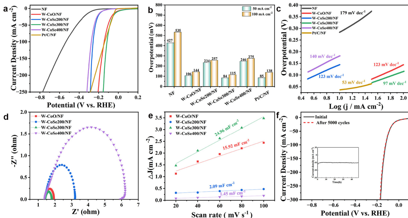
Fig. 4 HER performance: (a) LSV curves, (b) the corresponding overpotential at a current density of 50 \text{ mA cm}^{-2} ( \eta_{50} ) and 100 \text{ mA cm}^{-2} ( \eta_{100} ). (c) Tafel plots, (d) EIS Nyquist diagram, (e) C_{dl} values of different electrocatalysts, and (f) electrochemical stability tests of W-CoSe300/NF.
