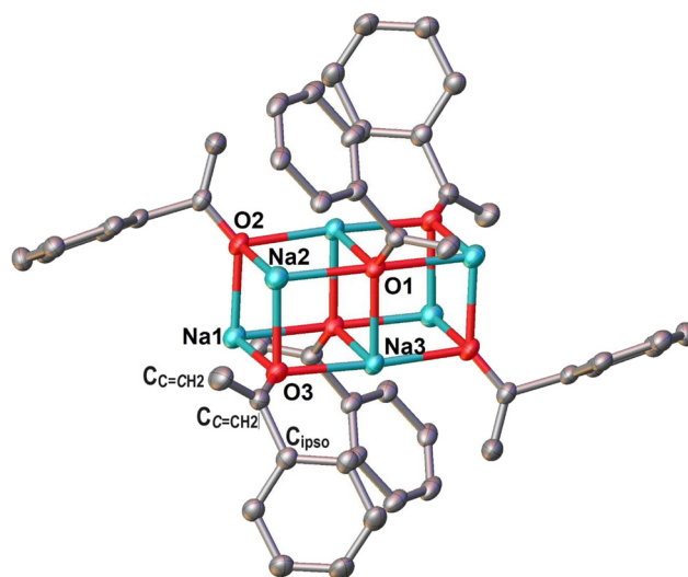
Fig. 3 The SCXRD structure of 3-Na. Hydrogen atoms, solvent benzene molecules in the lattice, and the two flanking phenyl rings of the anthracene are omitted for clarity. Half of the whole molecule is crystallographically independent, while the key independent atoms are labelled. Key bond lengths are provided as ranges: \text{Na-O} (2.24–2.38 Å), \text{O-C}=\text{CH}_2 (1.32–1.33 Å), \text{C}=\text{CH}_2\text{-C}=\text{CH}_2 (1.33–1.34 Å), \text{C}=\text{CH}_2\text{-C}_{\text{ipso}} (1.49–1.51 Å).
