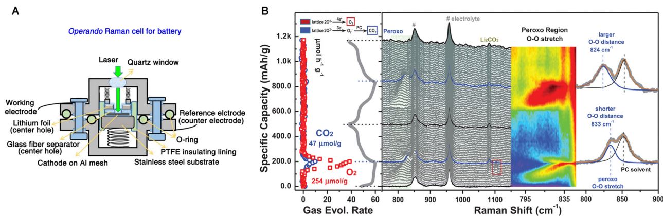
Fig. 13 (A) Schematic of an operando Raman cell for Li-ion batteries. (B) Operando Raman spectra and DEMS of the gas evolution rate during the first and second cycle of a \text{Li}_{0.6}[\text{Li}_{0.2}\text{Mn}_{0.8}]\text{O}_2 cathode in an electrolyte consisting of 1 M \text{LiClO}_4 in propylene carbonate. The peaks marked by the number sign at \sim 850 and 920\text{ cm}^{-1} originate from the electrolyte. Fig. 13A is reproduced with permission from ref. 153. Copyright 2018 the Royal Society of Chemistry. Fig. 13B is reproduced with permission from ref. 150. Copyright 2020 John Wiley and Sons.
