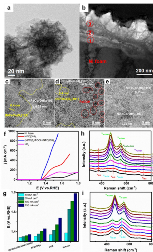
Fig. 8 Electro-oxidation of urea by (NiFeCo) x /FeOOH/NiFeCo(OH) x : (a) top-view and (b) cross-sectional TEM images of the electrocatalyst, HRTEM images of (c) the bottom layer, (d) middle layer, and (e) top layer in (b); comparison of different catalysts for urea electrooxidation: (f) the relevant polarization LSV curves and (g) the potential at different current densities; and operando Raman spectra of (h) (NiFeCo) x /FeOOH/NiFeCo(OH) x and (i) NiFeCo(OH) x . 5
