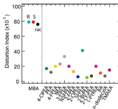
Fig. 23 D values of (R/S/Rac-MBA)_2SnI_4 and of other Sn-I layered HOIPs reported in the literature. Reprinted with permission from ref. 42 Copyright©2020 American Chemical Society.
