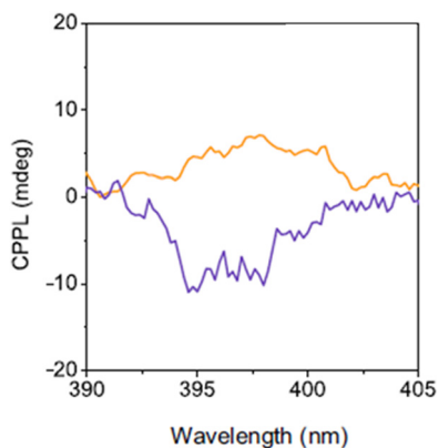
Fig. 20 CPL spectra of (R-NPB)_2PbBr_4 (orange curve) and (R-NEA)_2PbBr_4 (violet curve). Reprinted with permission from ref. 39 Copyright©2023 Nature Publishing Group.
