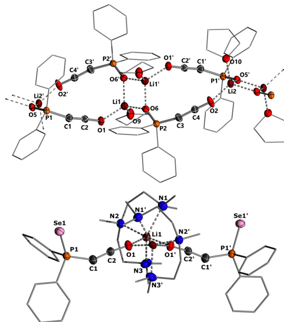
Fig. 4 Crystal structure of (top) 3a-Li and (bottom) 3c-Li (PMDETA). Ellipsoids are drawn at the 50% probability level. Important bond lengths [Å] and angles [ ^\circ ]: 3a-Li : P1–C1 1.677(4), C1–C2 1.230(6), C2–O1 1.216(5), P1–O1 1.510(3), P1–C1–C2 161.9(4), C1–C2–O1 176.7(5), P2–C3 1.673(4), C3–C4 1.231(6), C4–O2 1.206(5), P2–O6 1.509(3), P2–C3–C4 162.4(4), C1–C2–O1 176.7(5). 3c-Li (PMDETA): P1–Se1 2.132(1), P1–C1 1.698(6), C1–C2 1.243(8), C2–O1 1.222(7), O1–Li1 2.069(10), P1–C1–C2 147.8(5), C1–C2–O1 173.9(6).
