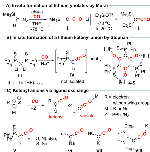
Fig. 1 (A) In situ formation of a lithium ynoate by carbonylation of metalated a diazomethane. (B) Formation of ketenyl anion from the reaction of a dilithiomethandiide with CO and N 2 O or (C) via PPh 3 /CO exchange and examples of isolated ketenyl anions.
