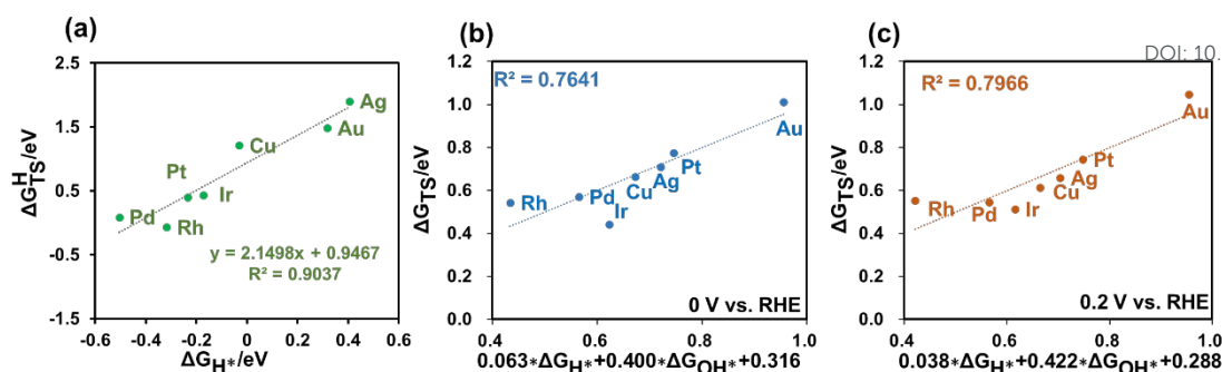
Fig. 3. linear relationships between the activation energy of the primary reaction steps and descriptors. (a) The linear relationship between H_2 dissociation barrier and H adsorption energy. (b, c) The relationship between the activation energy of the Direct Volmer step and the calculated adsorption energy of H and OH in (b) 0V vs. RHE and (c) 0.2V vs. RHE, the linear fit formula is expressed as the axis label, respectively.
