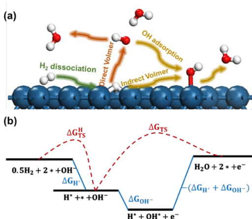
Fig. 1. (a) The reaction processes considered in the current work; (b) A schematic free energy diagram depicting the reaction steps. \Delta G_{\text{H}^*} and \Delta G_{\text{OH}^*} represent the adsorption energy of H and OH - , respectively. \Delta G_{\text{TS}}^{\text{H}} and \Delta G_{\text{TS}} represent the activation energy of H 2 dissociation and the Direct Volmer step. Blue, red, and white balls indicate Pt, O, and H, respectively.
