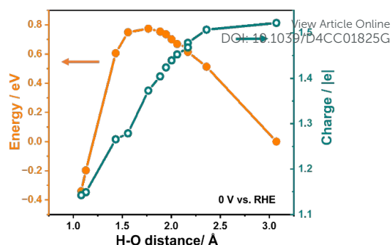
Fig. 2. Variation in system energy and the relative charge during the simulation of the Direct Volmer step on Pt(111) under the condition of a constant electrode potential of 0 V vs RHE at different H-O distances.
