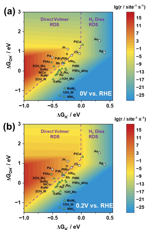
Fig. 4. Rate maps of HOR at (a) 0 V and (b) 0.2 V vs. RHE, constructed using H and OH adsorption energies as descriptors. Hollow pentagrams represent the seven pure metals, while green triangular markers denote additional computed alloy catalysts. Purple dashed lines delineate the rate maps into two distinct regions corresponding to different rate-determining steps.
