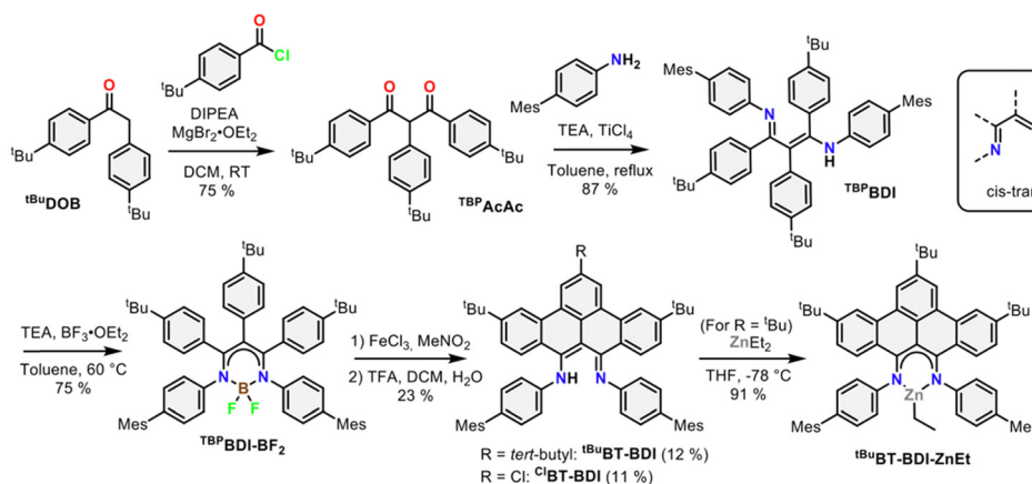
Scheme 1 Synthetic route towards {}^{\text{tBu}}\text{BT-BDI} and its ZnEt complex.
