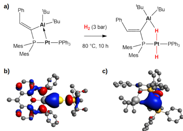
Fig. 5 (a) Experimentally reported reactivity of a Pt \rightarrow Al complex with \text{H}_2 . 52 (b) and (c) Isosurfaces of the HOMO of the gold-aluminy (b) and platinum-aluminy complex (c). The isovalue is 3 m_e a_0^{-3} . The isosurfaces have been taken and adapted with permission from ref. 50 Copyright 2023, Royal Society of Chemistry.
