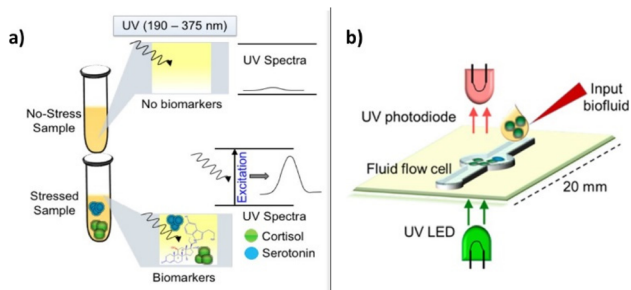
Fig. 4 Optical absorption approach for label-free biomarker detection: (a) basic absorption function; (b) integration approach. Reproduced from ref. 70 with permission from American Chemical Society, copyright 2019.
