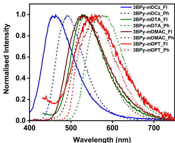
Fig. 3 Fluorescence (FI) and phosphorescence (Ph) spectra of 7 wt% 3BPpy-mDCz :DPEO, 3BPpy-mDTA :mCBP, 3BPpy-mDMAC :mCBP and 3BPpy-mDPT :mCBP doped film.
