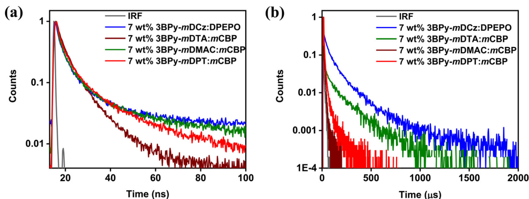
Fig. 4 Transient PL decays of DPEPO and mCBP host films doped with 7 wt% of emitter (a) prompt and (b) delayed component at 298 K.
