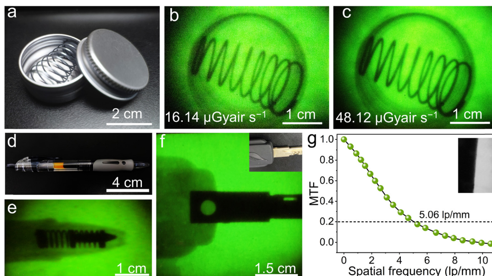
Fig. 6 (a) Photograph of aluminum specimen box with an iron spring under visible light. (b) and (c) X-ray imaging of an aluminum specimen box with an iron spring under the X-ray doses of 16.14 \mu\text{Gy}_{\text{air}} \text{ s}^{-1} and 48.12 \mu\text{Gy}_{\text{air}} \text{ s}^{-1} , respectively. (d) Photograph of the ball-point pen. (e) X-ray imaging of the ball-point pen under the X-ray dose of 16.14 \mu\text{Gy}_{\text{air}} \text{ s}^{-1} . (f) X-ray imaging of a metallic key partially wrapped in rubber under the X-ray dose of 16.14 \mu\text{Gy}_{\text{air}} \text{ s}^{-1} , inset shows the photograph of the same metallic key. (g) MTF of the \text{Cs}_2\text{ZnBr}_4\text{:25\%Mn}^{2+} thin film scintillation screen measured by the slanted-edge method (inset).
