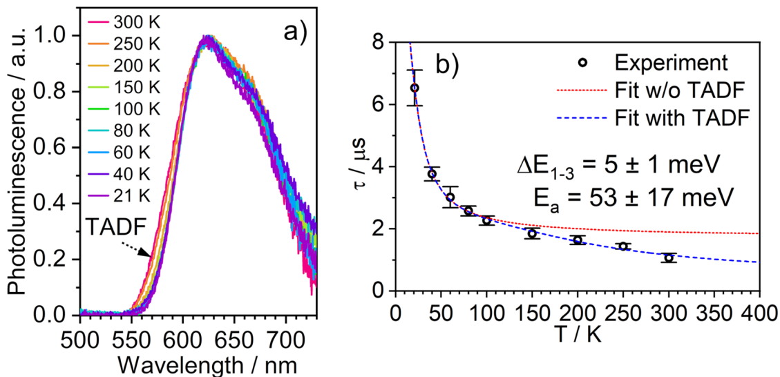
Fig. 5 (a) The PL spectra of 1 in polystyrene matrix at (0.1% w/w) at the temperatures indicated. (b) The corresponding variation in \tau_{\text{obs}} . The experimental data points are represented by black circles and the best fit to eqn (2) by the dashed blue line. The corresponding "fit" in the absence of the TADF component is shown by the dotted red line. \lambda_{\text{ex}} = 355 nm.
