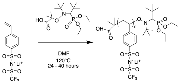
Fig. 1 Nitroxide mediated polymerization of STFSI-Li.
