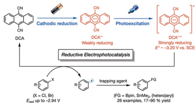
Scheme 6 Reductive electrophotocatalysis with the photoexcited state of DCA •- (*DCA •- ) for the reductive borylation of aryl chlorides and aryl bromides with bis(pinacolato)diboron (B 2 pin 2 ). Reprinted from ref. 42 with permission from American Chemical Society (Copyright 2010).
