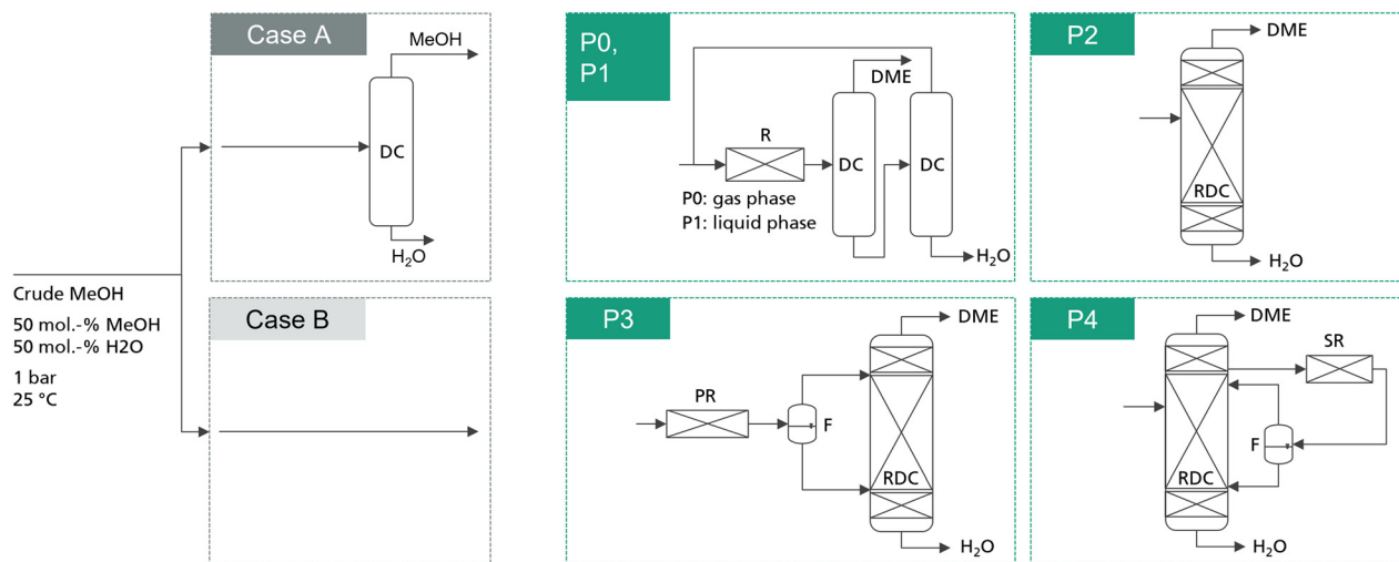
Fig. 1 Simplified process flowsheets of the examined process concepts. Detailed flowsheets are presented in the ESI† P1–P4 are studied for the case of integrating a dedicated crude MeOH distillation column (case A) and for the case of feeding crude MeOH directly into the respective DME process (case B). The conventional process P0 is only analysed including the crude MeOH distillation column.
