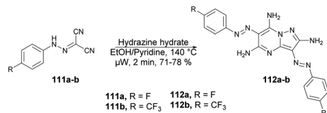
Scheme 39 Synthesis of diarylazo-2,5,7-triaminopyrazolo[1,5-a]pyrimidines 112a-b .
