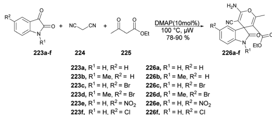
Scheme 79 Synthesis of spiro-4H-pyrans 226a–f .
