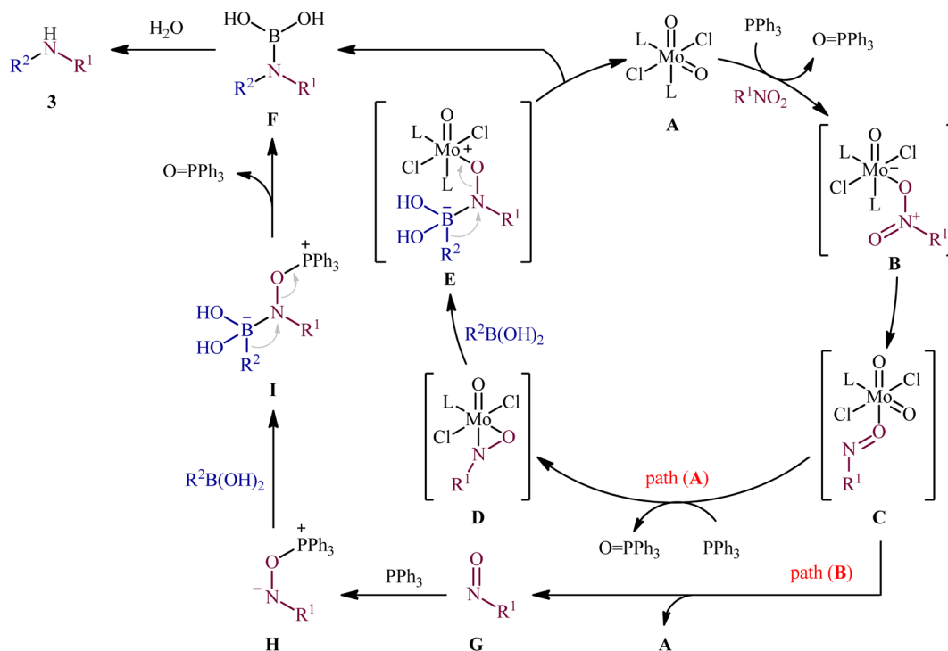
Scheme 3 Mechanism that accounts for the formation of secondary amines 3 .
