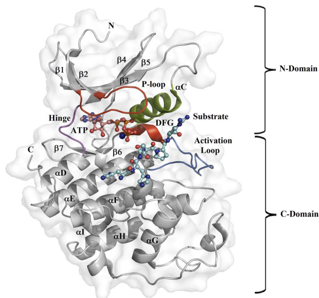
Fig. 1 Design of the PK catalytic domain. The structural topology of a PK exemplified by CDK2 (PDB entry 1QM2). The figure illustrates the N- and C-domains of CDK2, which forms a complex with ATP and the substrate at the catalytic binding domain. The activation loop is in blue, the P-loop in red, the \alpha C-helix in green, the hinge region in magenta, the Mg^{2+} ion in orange, the ATP in pink, and the substrate in cyan.
