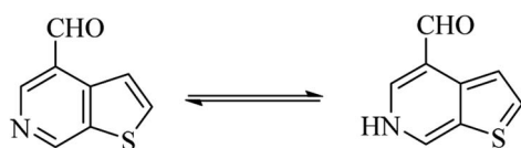
Fig. 25 Tautomers of thieno-pyridine carbaldehyde.
