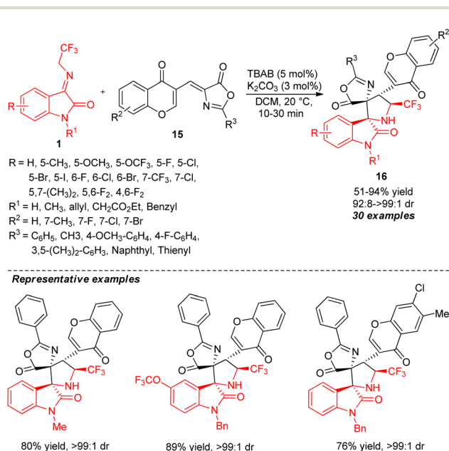
Scheme 7 TBAB-catalyzed highly diastereoselective [3+2] cycloaddition of ketimines to access spirooxindoles.
