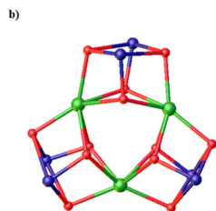
Fig. 1 Crystal structure of R -1; all H atoms and solvent molecules are omitted for clarity (a). Corner-sharing [\text{Cu}_6\text{Dy}_3(\text{R-L})_6(\text{OH})_6] cubanes (b).
