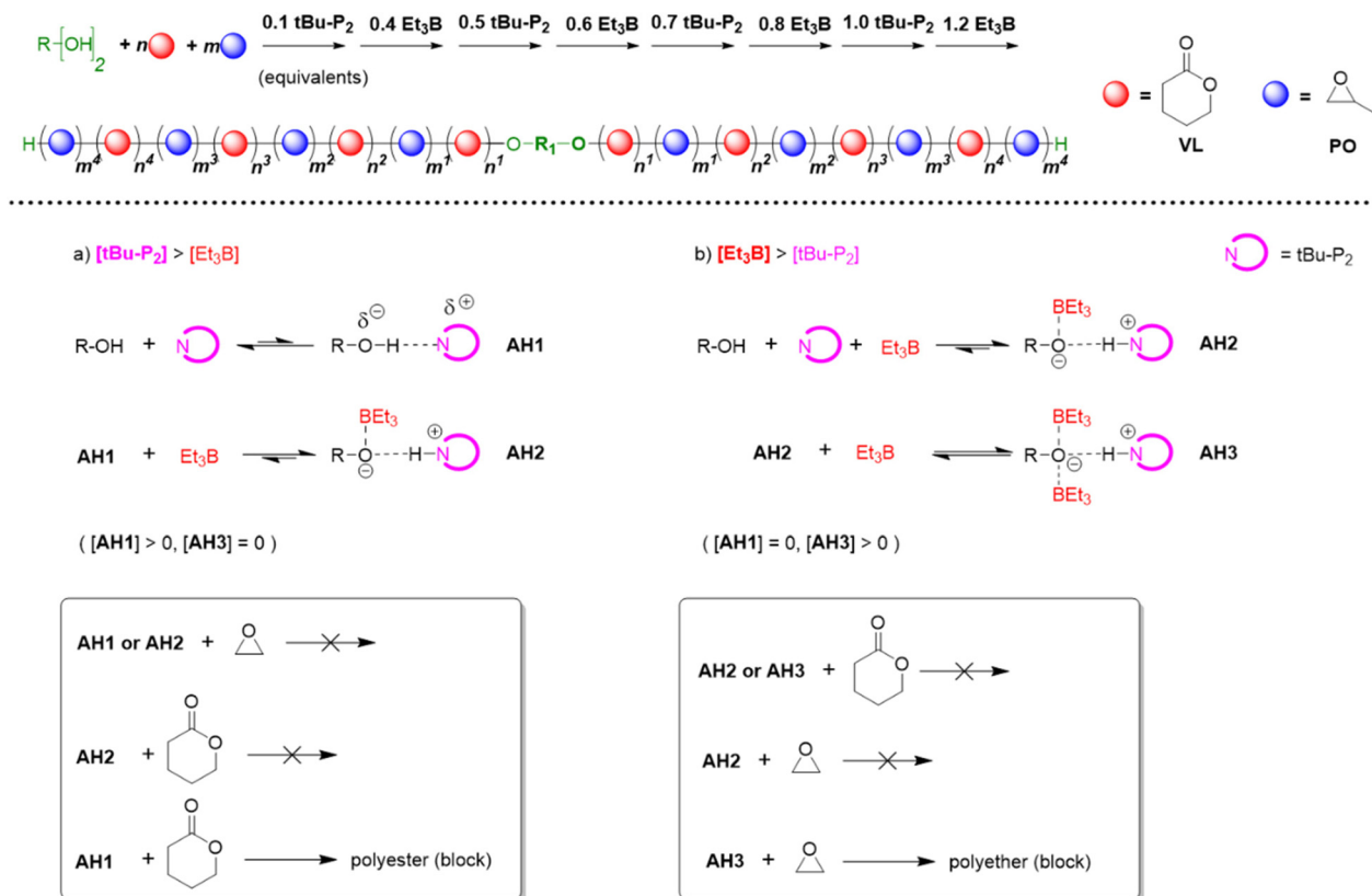
Scheme 10 Top: using the \text{Et}_3\text{B} /organobase stoichiometry to synthesize well-defined poly(ester-ether) multiblock copolymers. Bottom: different species of activated hydroxyl and respective selectivity.
