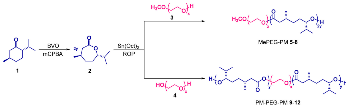
Scheme 1 ROP of (–)-menthicide catalyzed by stannous octoate in the presence of PEG-based macroinitiators.
