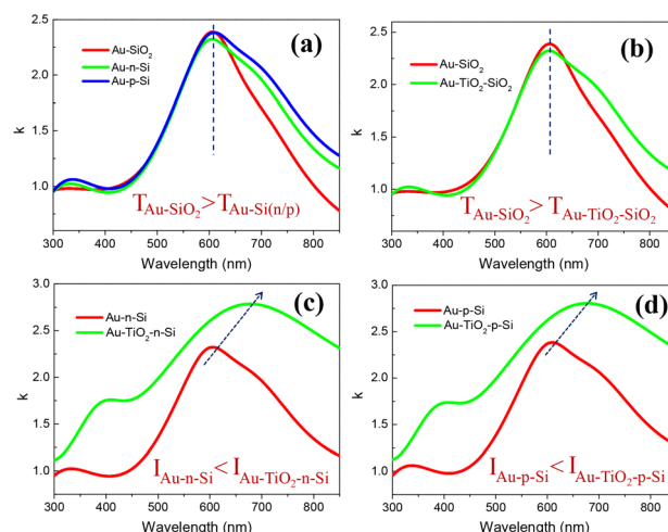
Fig. 3 Extinction coefficient of Au particles for different samples. (a) Au-SiO 2 , Au-n-Si and Au-p-Si, (b) Au-SiO 2 and Au-TiO 2 -SiO 2 , (c) Au-n-Si and Au-TiO 2 -n-Si, and (d) Au-p-Si and Au-TiO 2 -p-Si.
