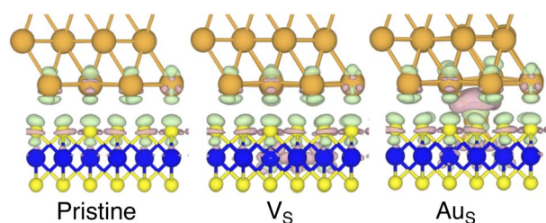
Fig. 4 Electron density difference (EDD) maps of the pristine, V_S , and \text{Au}_5 interfaces in the vicinity of the contact area. Green colour corresponds to electron loss, whereas mauve colour to electron enrichment. The isovalue was set to 0.002 \text{ eV } \text{\AA}^{-3} .
