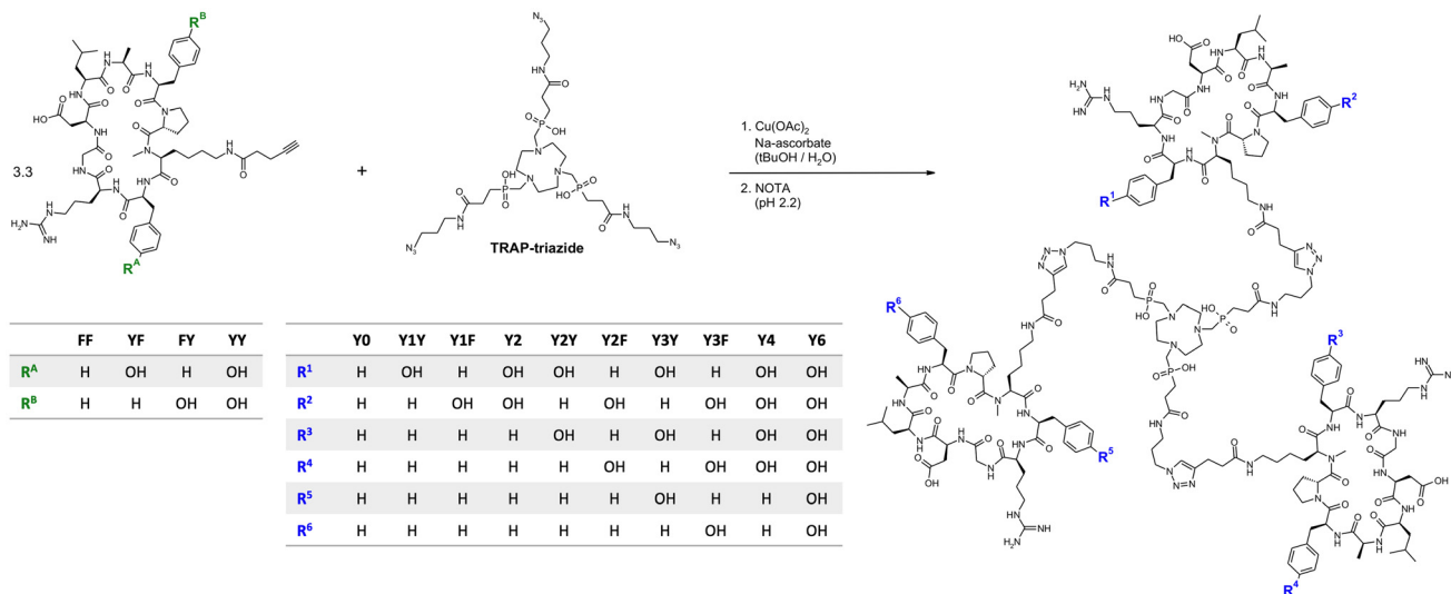
Fig. 1 Synthesis of trimeric conjugates of \alpha\text{v}\beta 6 -integrin binding peptides. Synthesis of Y0 , Y3Y , Y3F , and Y6 was done by reacting TRAP-triazide with the peptides FF , YF , FY , and YY , respectively. For the remaining conjugates, the CuAAC reaction was done using 1 : 1 mixtures of two different peptides ( FF & YF , FF & FY , and FF & YY ), leading to statistical mixtures of the respective hetero-conjugates which were separated by preparative HPLC.
