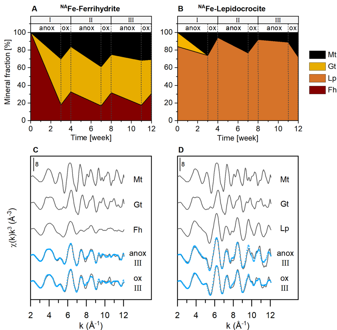
Fig. 2 Iron mineral fractions as determined by linear combination fitting of Fe K-edge EXAFS spectra in ^{NA}\text{Fe} -mineral samples from mesh bags without soil for (A) ^{NA}\text{Fe} -ferrihydrate and (B) ^{NA}\text{Fe} -lepidocrocite incubated for 12 weeks in the redox fluctuating mesocosms, with (C and D) reference spectra and spectra from redox cycle III. According to EXAFS data, the initial ^{NA}\text{Fe} -lepidocrocite contained minor fractions (16%) of goethite which was likely nano-crystalline (ESI Section S2†). All spectra and fits are presented in Fig. S15.† Fractions of fit components and reduced \chi^2 are presented in Table S4.† Abbreviations: Mt = magnetite, Gt = goethite, Fh = ferrihydrite, Lp = lepidocrocite, anox = anoxic, ox = oxic.
