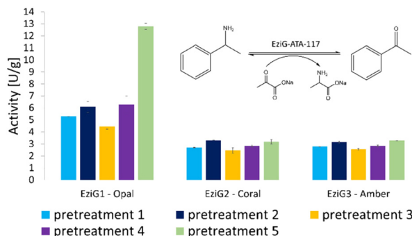
Fig. 3 Enzymatic activity (expressed in enzymic unit per g of immobilized enzyme) of the immobilized His 6 -ATA-117 formulations on EziG 1 -Opal, EziG 2 -Coral, and EziG 3 -Amber pre-treated according to the protocols of Table 1. Reaction conditions: 100 mM HEPES pH 9.0, 10 mM sodium pyruvate, 20 mM \alpha -MBA, 25 °C, 15 rpm, 15 min. The formation of acetophenone was monitored by measuring the increase in absorbance at 245 nm (see the scheme in the inset of the figure). Immobilization yields: 92.4% EziG 1 -Opal, 92.5% EziG 2 -Coral and 92.2% EziG 3 -Amber.
