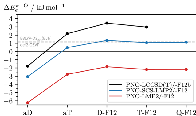
Fig. 9 Comparison of PNO (with aX≡aVXZ) and PNO-F12 (with X-F12≡VXZ-F12) predictions of the relative electronic stabilities of c2NA_O and c2NA_\pi ( \Delta E_e^{\pi-O} ) for increased coverage of the one-particle basis space. The optimised B3LYP-D3 abc (BJ)/def2-QZVP geometries are used (reference values shown in grey).
