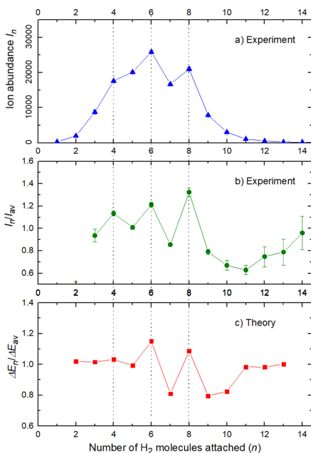
Fig. 5 Data for \text{Na}^+(\text{H}_2)_n . Panel a: experimental ion abundance versus size, n . Panel b: experimental ion abundance I_n divided by its local average, I_{av} . Panel c: evaporation energy \Delta E_n calculated with the rigid rotor model DMC, divided by its local average \Delta E_{av} . Note the similarity of the data in panels b and c.
