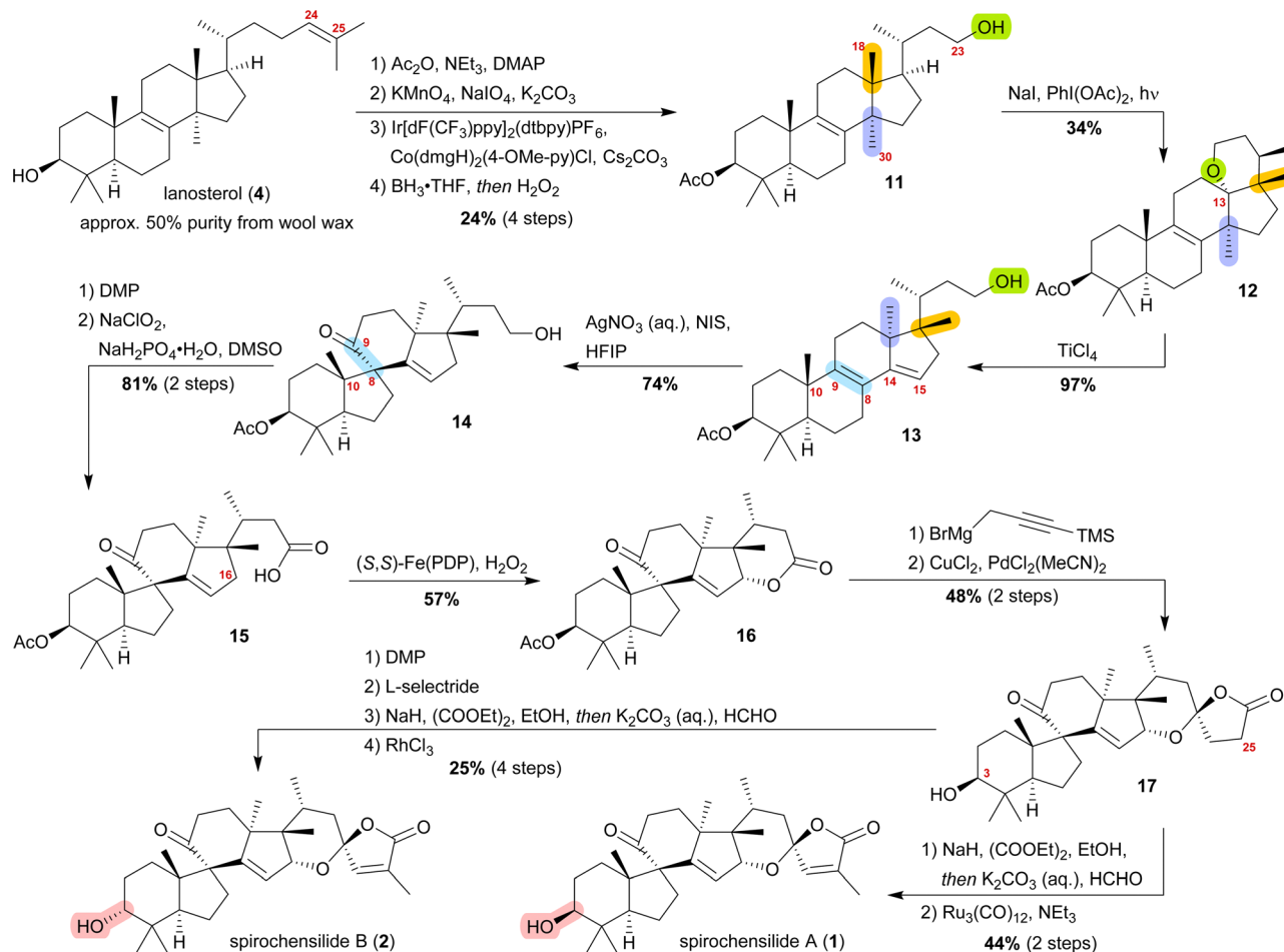
Scheme 2 Semisyntheses of spirochensilide A (1) and B (2) by Heretsch and co-workers. ppy = 2-phenylpyridine, dtbpy = 4,4'-di- t -butyl-2,2'-bipyridine, dmgH = dimethylglyoximato, ( S,S )-PDP = (–)-2-(( S )-2-(( S )-1-(pyridin-2-ylmethyl)pyrrolidin-2-yl)pyrrolidin-1-yl)methylpyridine.
