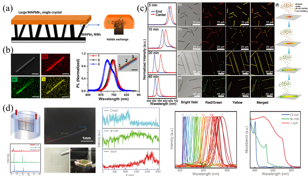
Fig. 10 (a) Schematic diagram of solid-phase ion exchange for HP NWs. (b) EDS mappings and PL spectra at different regions of compositional gradient \text{MAPbBr}_x\text{I}_{3-x} NWs. (a) and (b) Reprinted with permission from ref. 77, Copyright 2017, American Chemical Society. (c) PL spectra at the end and center of \text{CsPbBr}_x\text{I}_{3-x} NWs at different reaction times, and corresponding confocal laser scanning microscope image and schematic diagram of the growth process of compositional gradient \text{CsPbBr}_x\text{I}_{3-x} NWs. Reprinted with permission from ref. 89, Copyright 2018, John Wiley and Sons. (d) Schematic diagram of the dip-and-pull method for liquid-phase ion exchange for MWs, and corresponding characterization of the compositional gradient MWs. Reprinted with permission from ref. 41, Copyright 2022, John Wiley and Sons.
