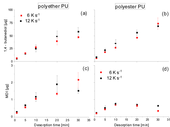
Fig. 3 Time-dependent thermal desorption at 250 ^{\circ}\text{C} of 1,4 butanediol and MDI from polyether PU (a and c) and polyester PU (b and d) at heating rates of 6 \text{K s}^{-1} (red) and 12 \text{K s}^{-1} (black).
