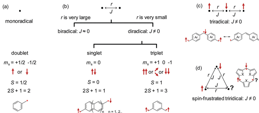
Fig. 1 Schematic graphs of a (a) monoradical, (b) biradical and diradical, (c) triradical, and (d) spin-frustrated triradical. r : the distance between two electrons; J : electron exchange integral; m_s : magnetic components; S : spin quantum number; (2S + 1) : spin multiplicity.
