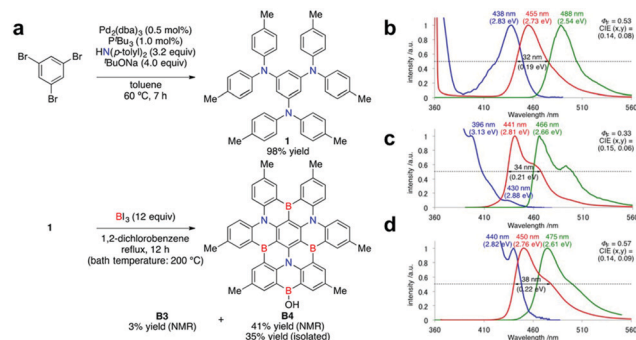
Fig. 12 (a) Two-step synthesis of B4. (b–d) Normalized absorption (blue), fluorescence (red), and phosphorescence (green, 77 K, 25 ms delay) spectra, with absorption/emission maxima, absolute fluorescence quantum yields ( \Phi_F ), and FWHM of PMMA films of B2, B3, and B4 (1 wt%, excited at 360 nm). Reprinted with permission from ref. 136. Copyright 2018 American Chemical Society.
