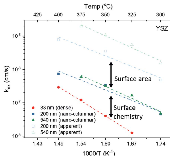
Fig. 10 Effect of nano-columnar growth on the surface exchange coefficient, k_{ex} , of L2NO4/YSZ: tailoring the microstructure from dense (33 nm) to nano-columnar (200 and 540 nm) leads to a significant enhancement of k_{ex} , due to modifications of the surface chemistry. The influence of the enlarged surface area is depicted using the apparent exchange coefficient, equivalent to the surface exchange coefficient required for a dense layer to exchange oxygen as fast as a nano-columnar one.
